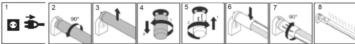
FIG. 8 SCHEMATIC STEPS OF REMOVING A FLUORESCENT LAMP AND INSERTING A DOUBLE-CAPPED LED LINEAR LAMP DESIGNED TO RETROFIT LINEAR FLUORESCENT LAMP
