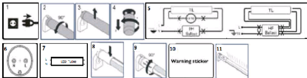
FIG. 9 SCHEMATIC STEPS OF REMOVING A FLUORESCENT LAMP AND INSERTING A DOUBLE-CAPPED LED LINEAR LAMP DESIGNED TO CONVERT LINEAR FLUORESCENT LAMP
