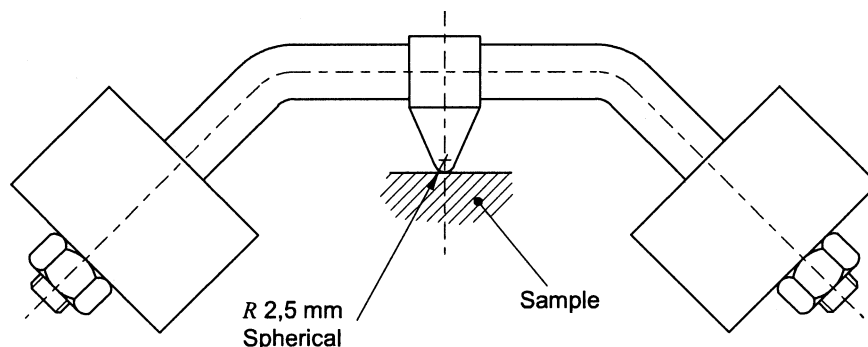
FIG. 12 BALL-PRESSURE TEST APPARATUS
